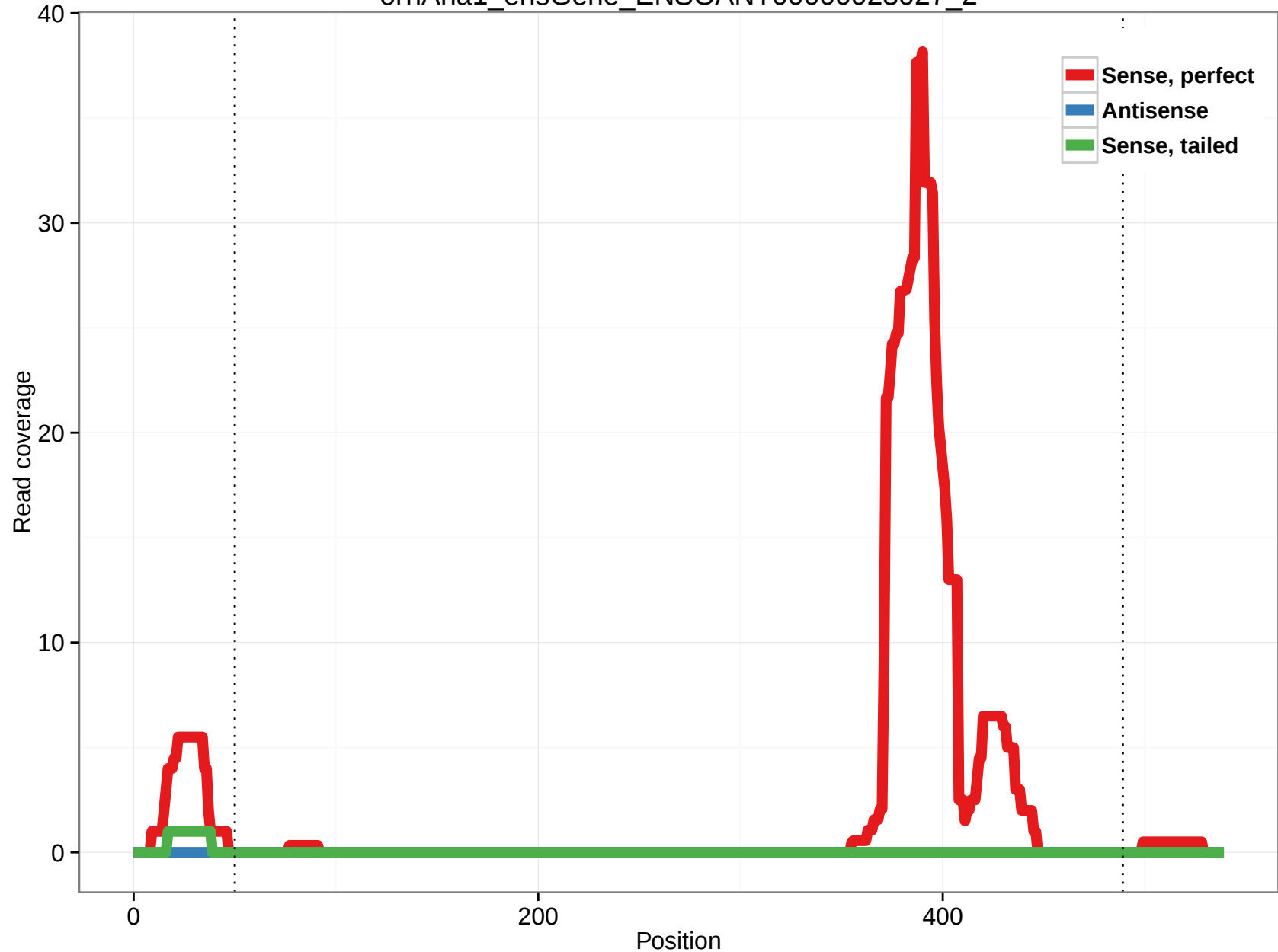
ornAna1_ensGene_ENSOANT00000023027_2
