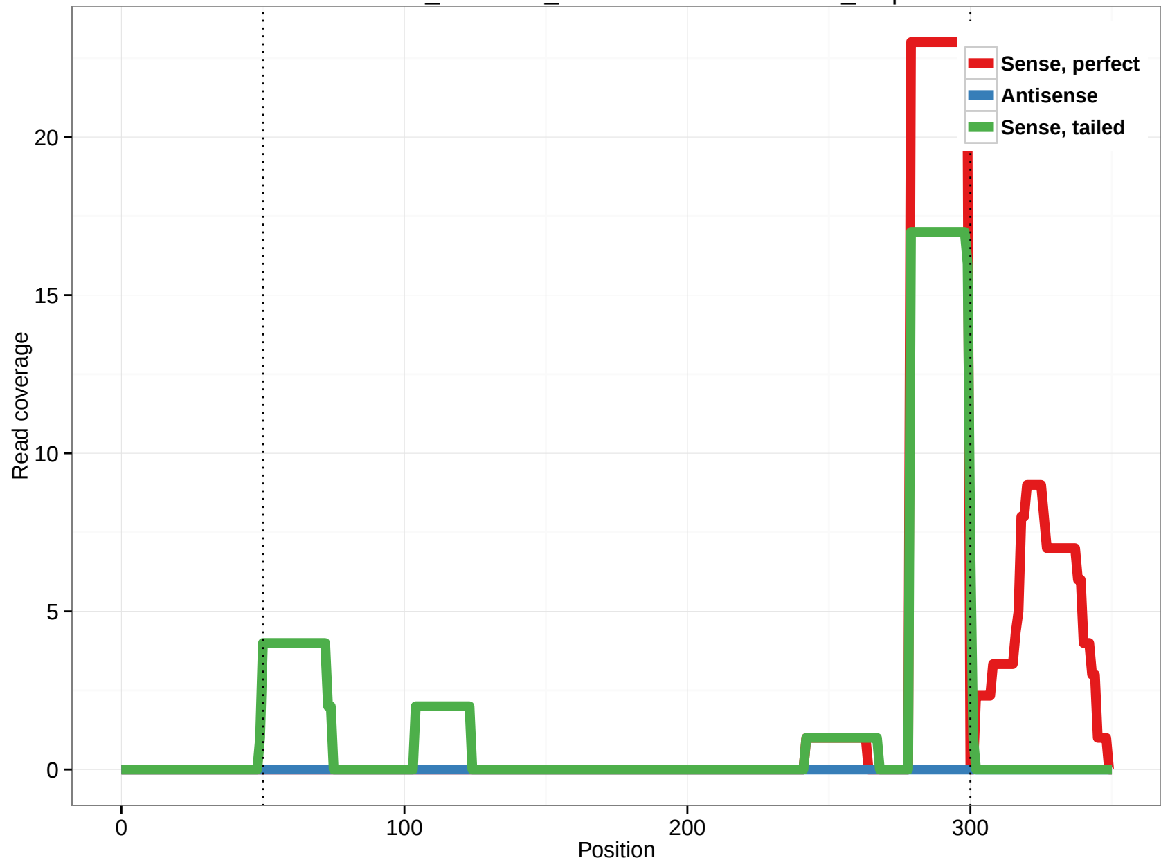
ornAna1_ensGene_ENSOANT00000022976_6.3p
