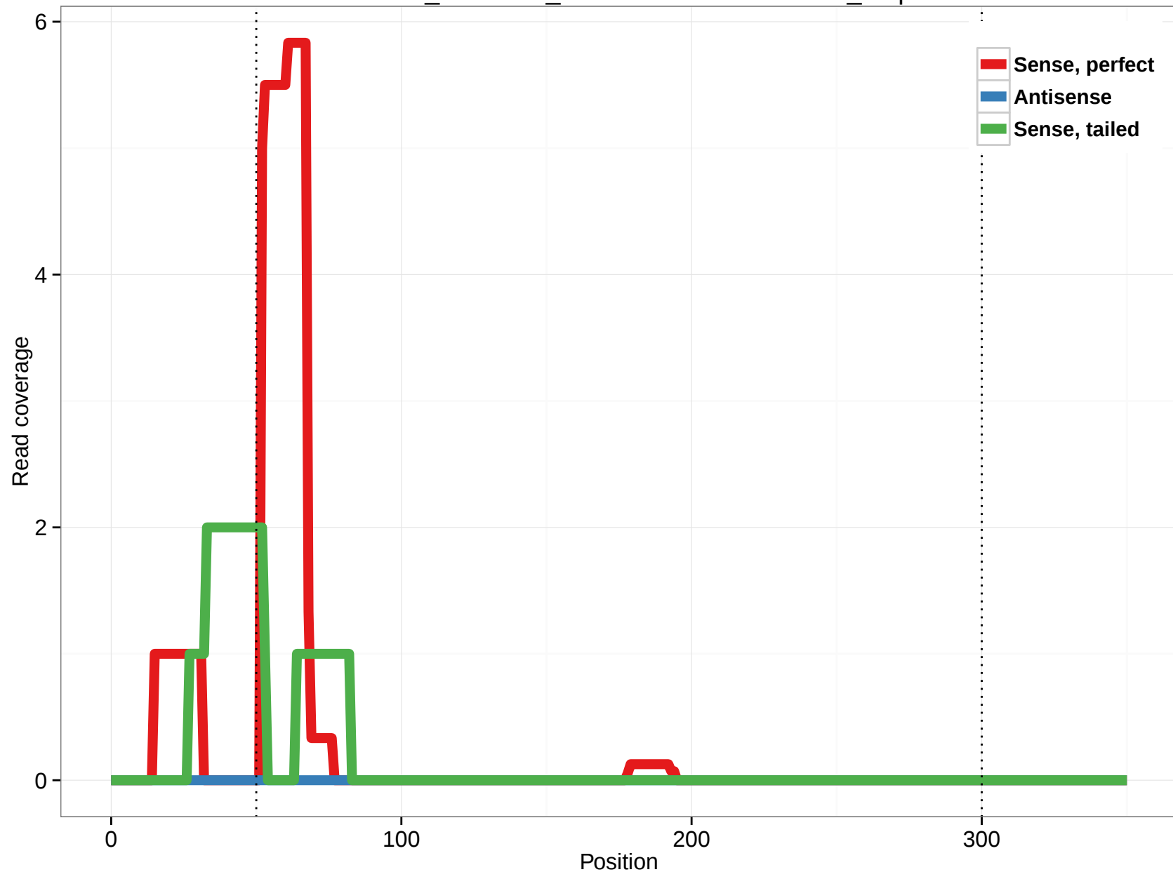
ornAna1_ensGene_ENSOANT00000022961_2.5p
