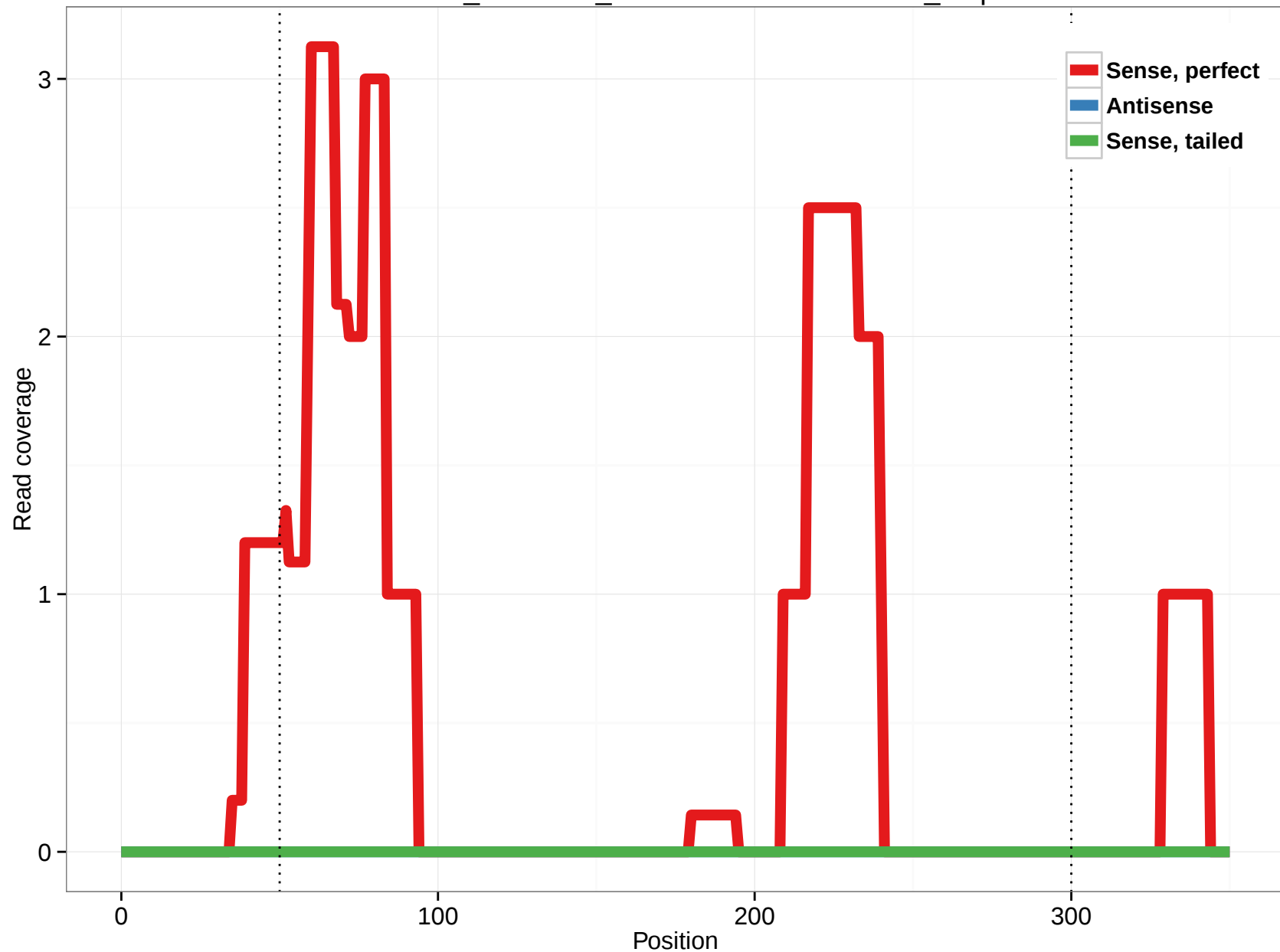
ornAna1_ensGene_ENSOANT00000022949_8.5p
