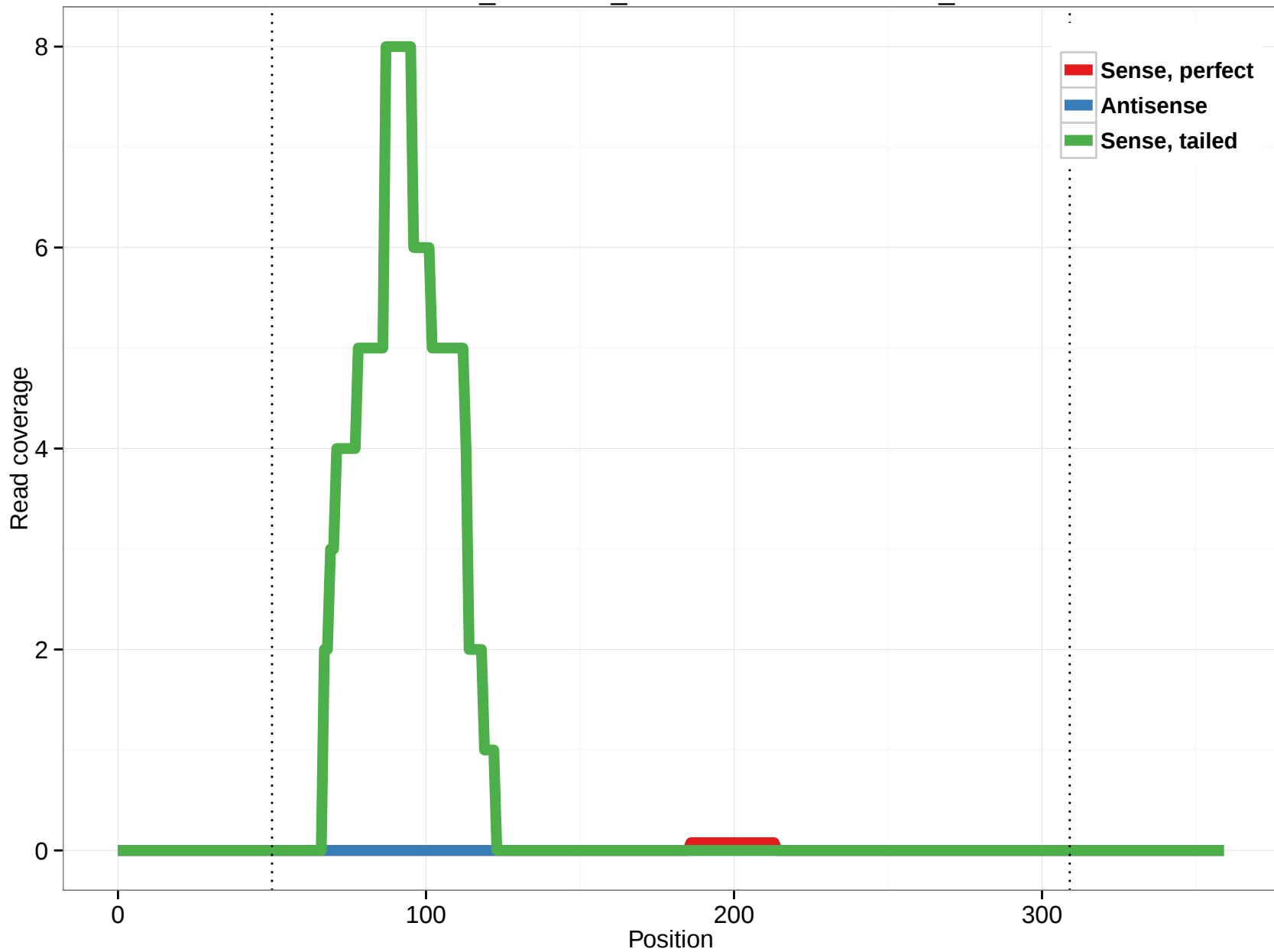
ornAna1_ensGene_ENSOANT00000022929_1
