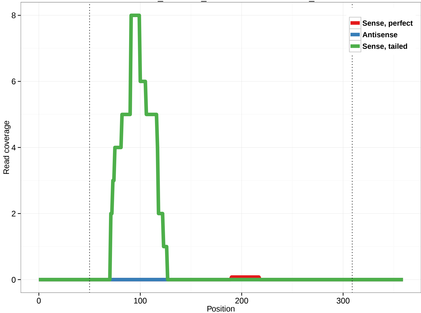
ornAna1_ensGene_ENSOANT00000022928_3
