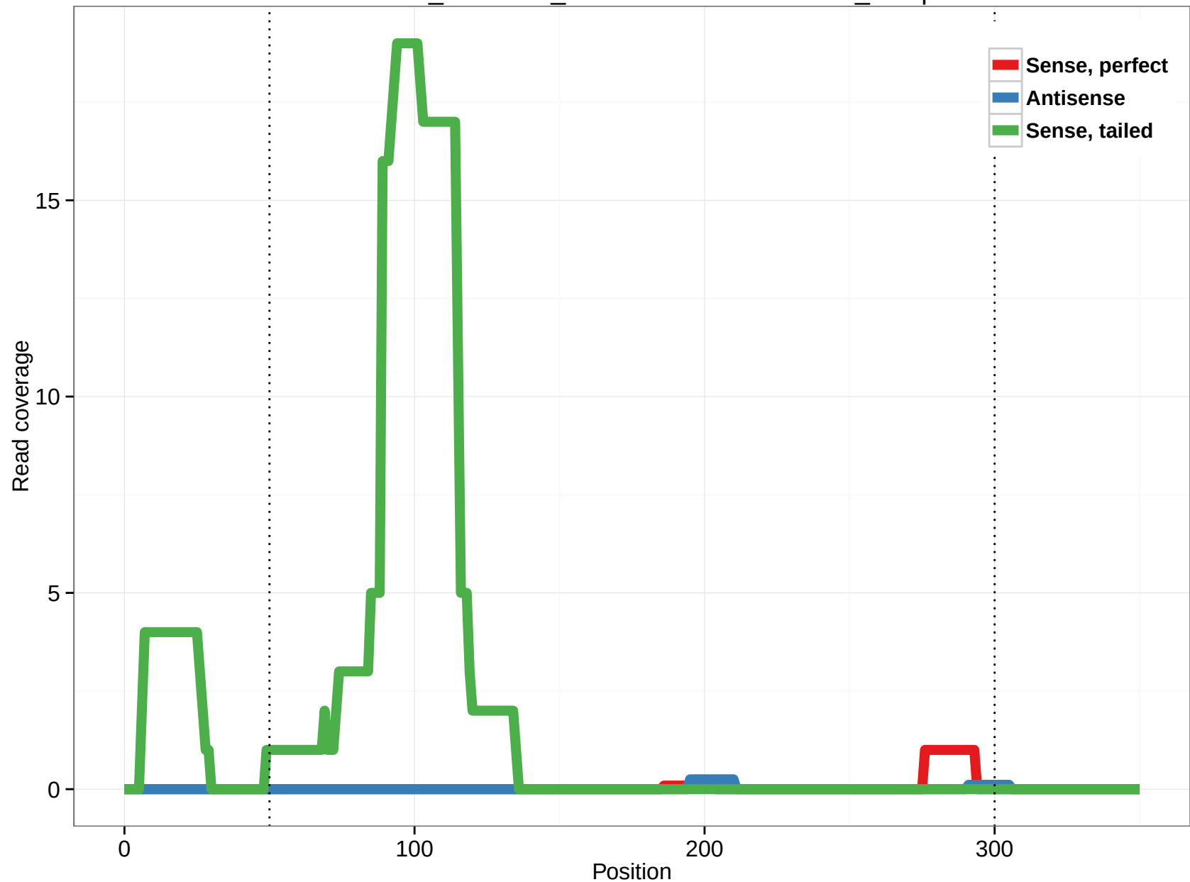
ornAna1_ensGene_ENSOANT00000022915_11.3p
