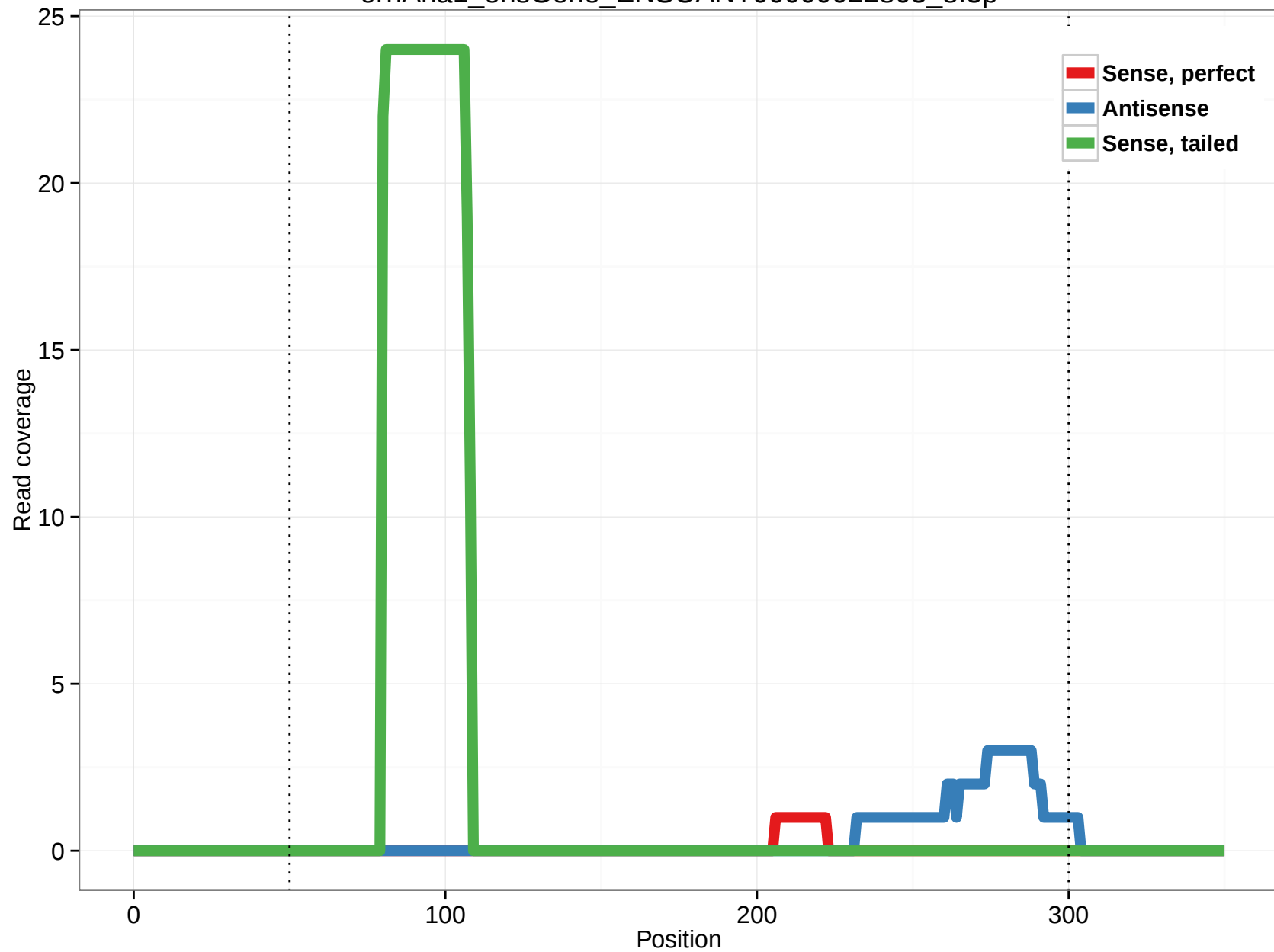
ornAna1_ensGene_ENSOANT00000022803_8.3p
