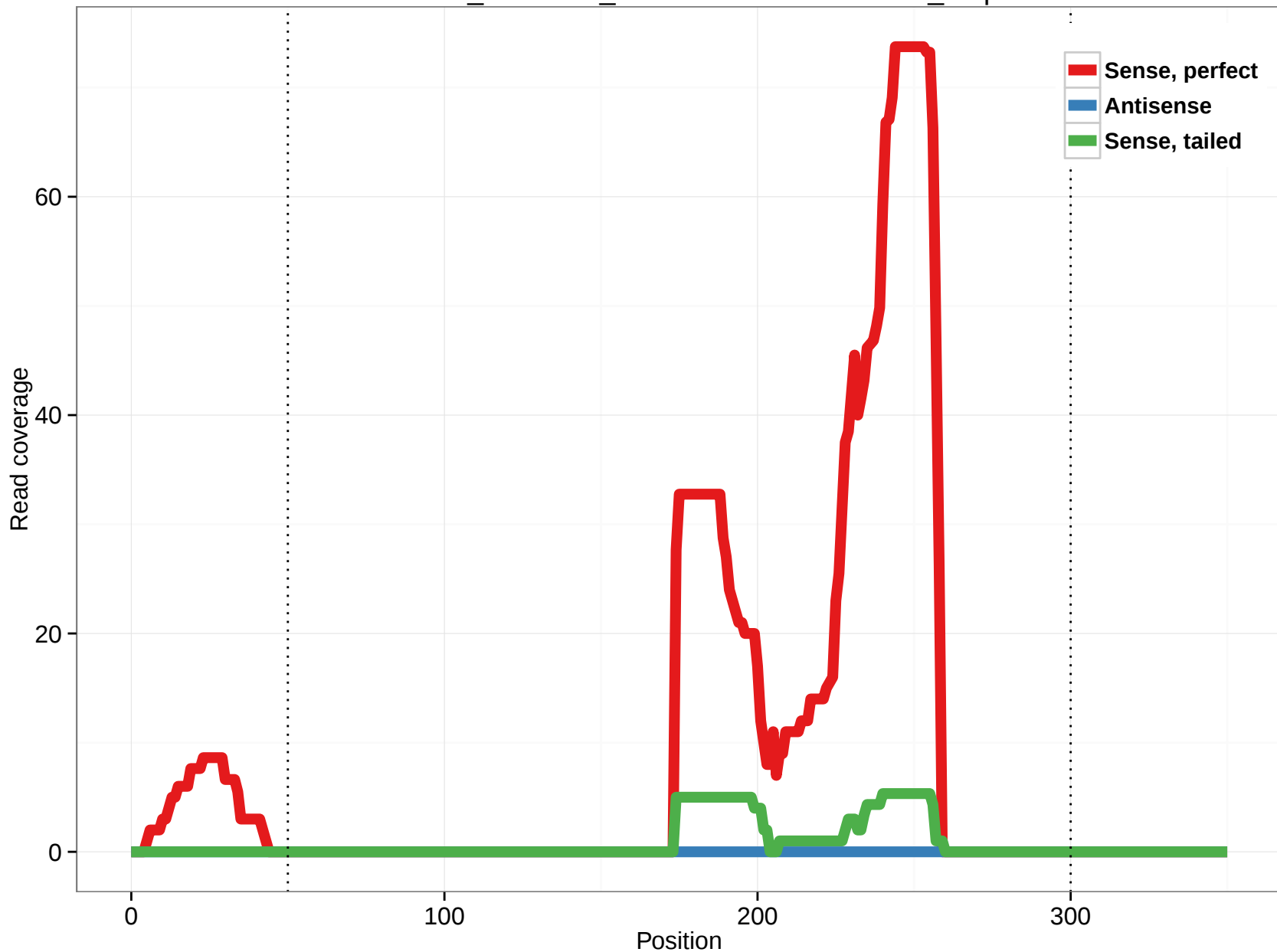
ornAna1_ensGene_ENSOANT00000022801_3.5p
