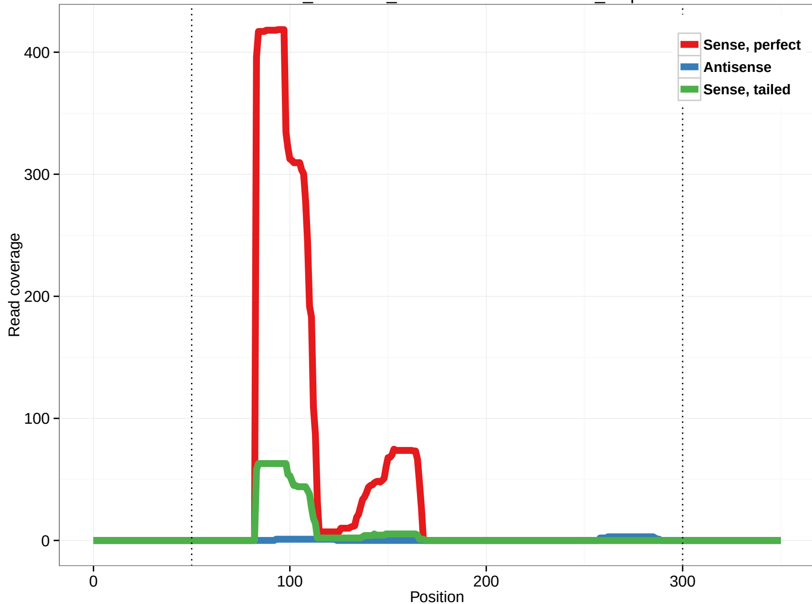
ornAna1_ensGene_ENSOANT00000022801_1.5p
