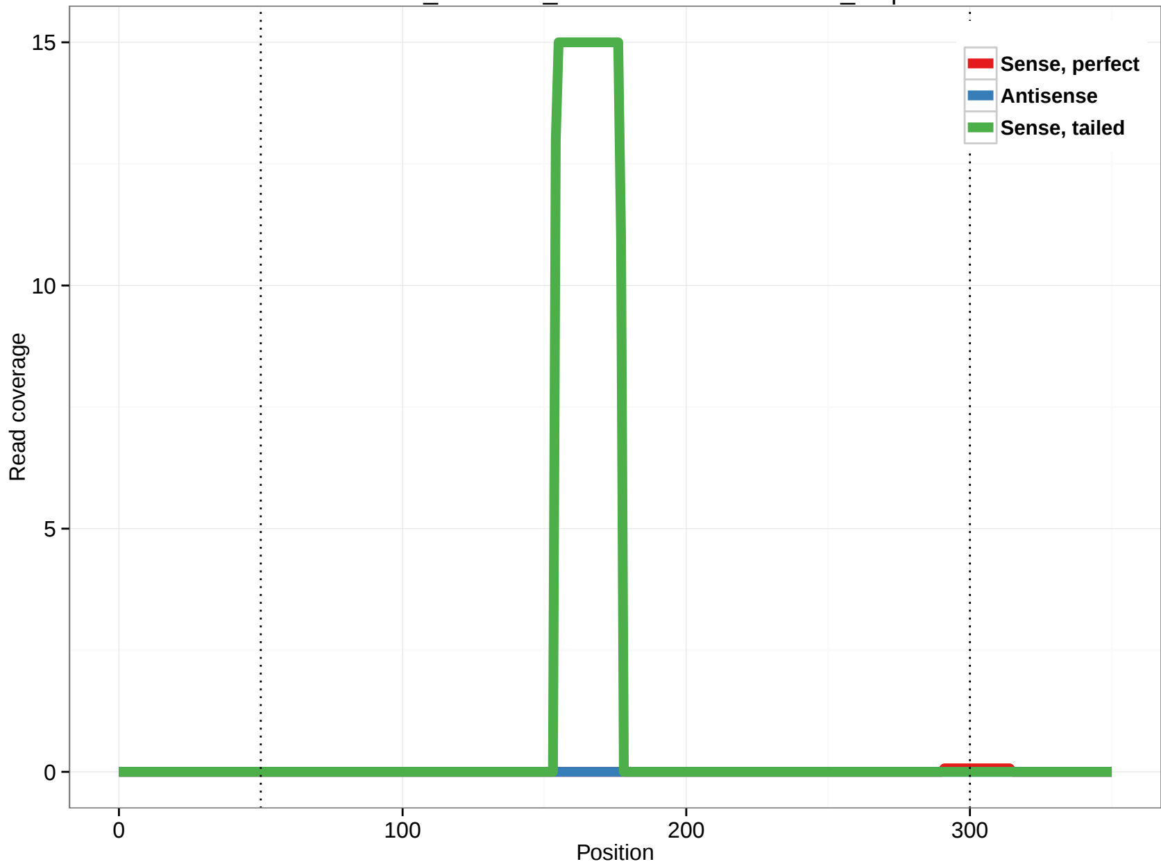
ornAna1_ensGene_ENSOANT00000022773_4.5p
