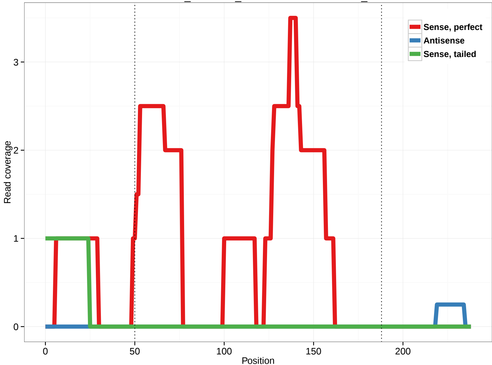
ornAna1_ensGene_ENSOANT00000022624_0
