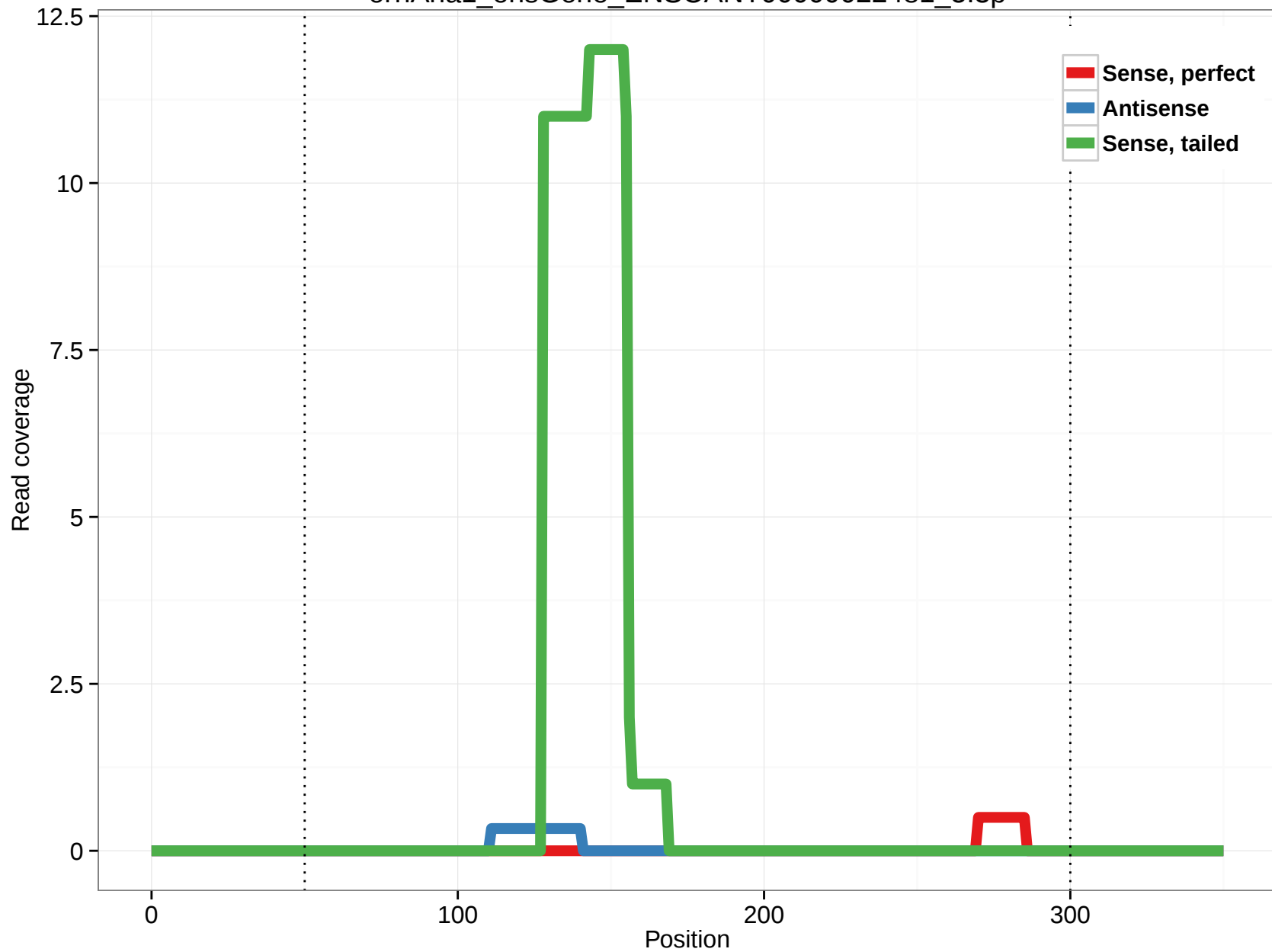
ornAna1_ensGene_ENSOANT00000022481_5.3p
