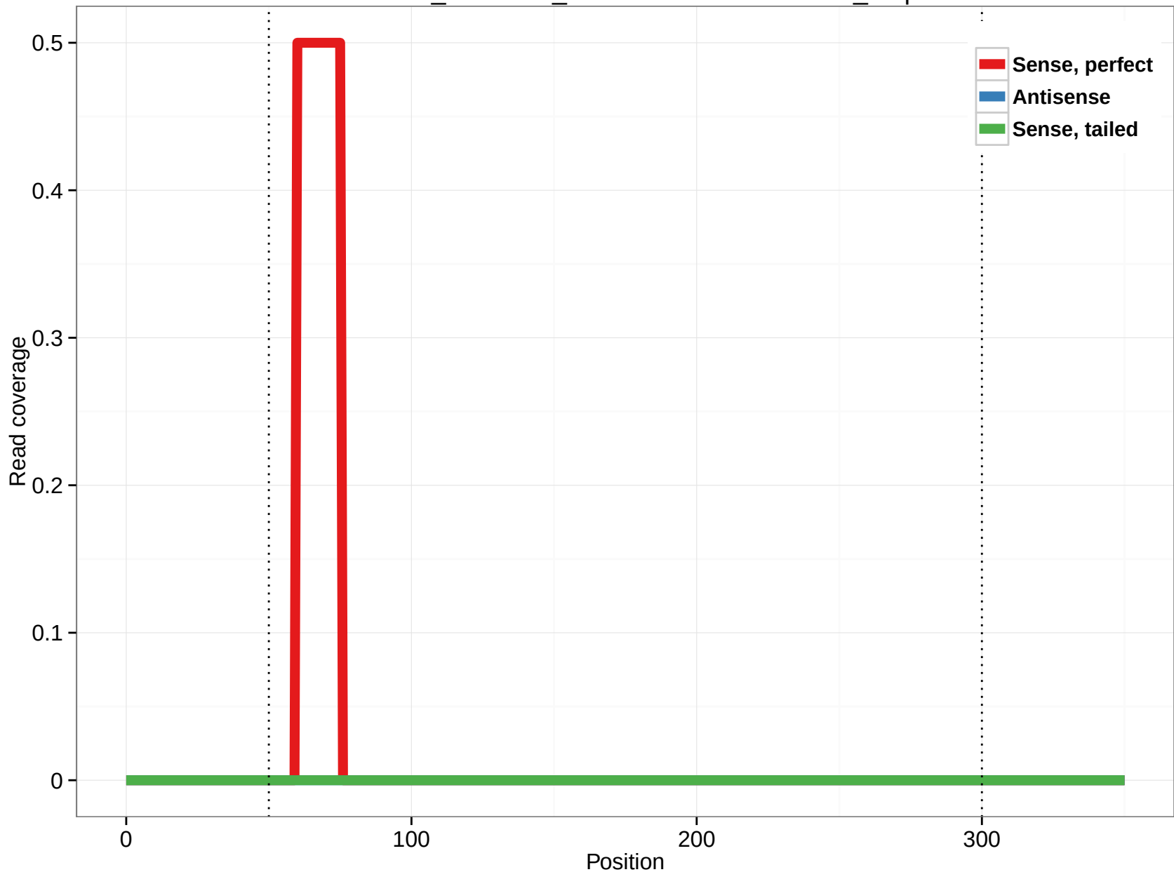
ornAna1_ensGene_ENSOANT00000022477_0.3p
