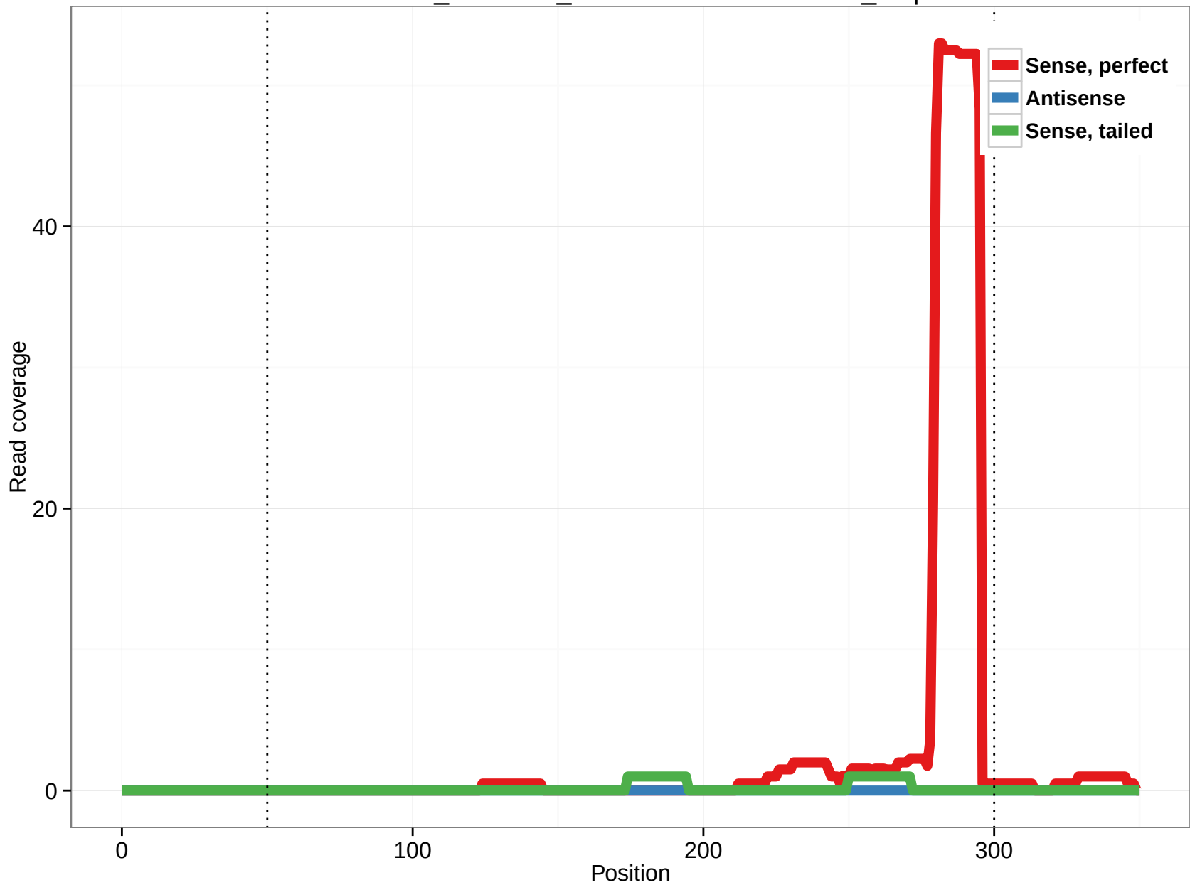
ornAna1_ensGene_ENSOANT00000022395_1.5p
