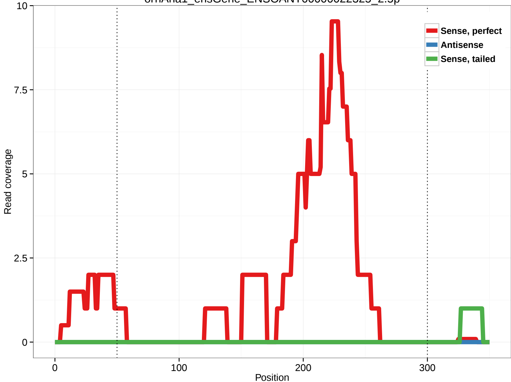
ornAna1_ensGene_ENSOANT00000022325_2.5p
