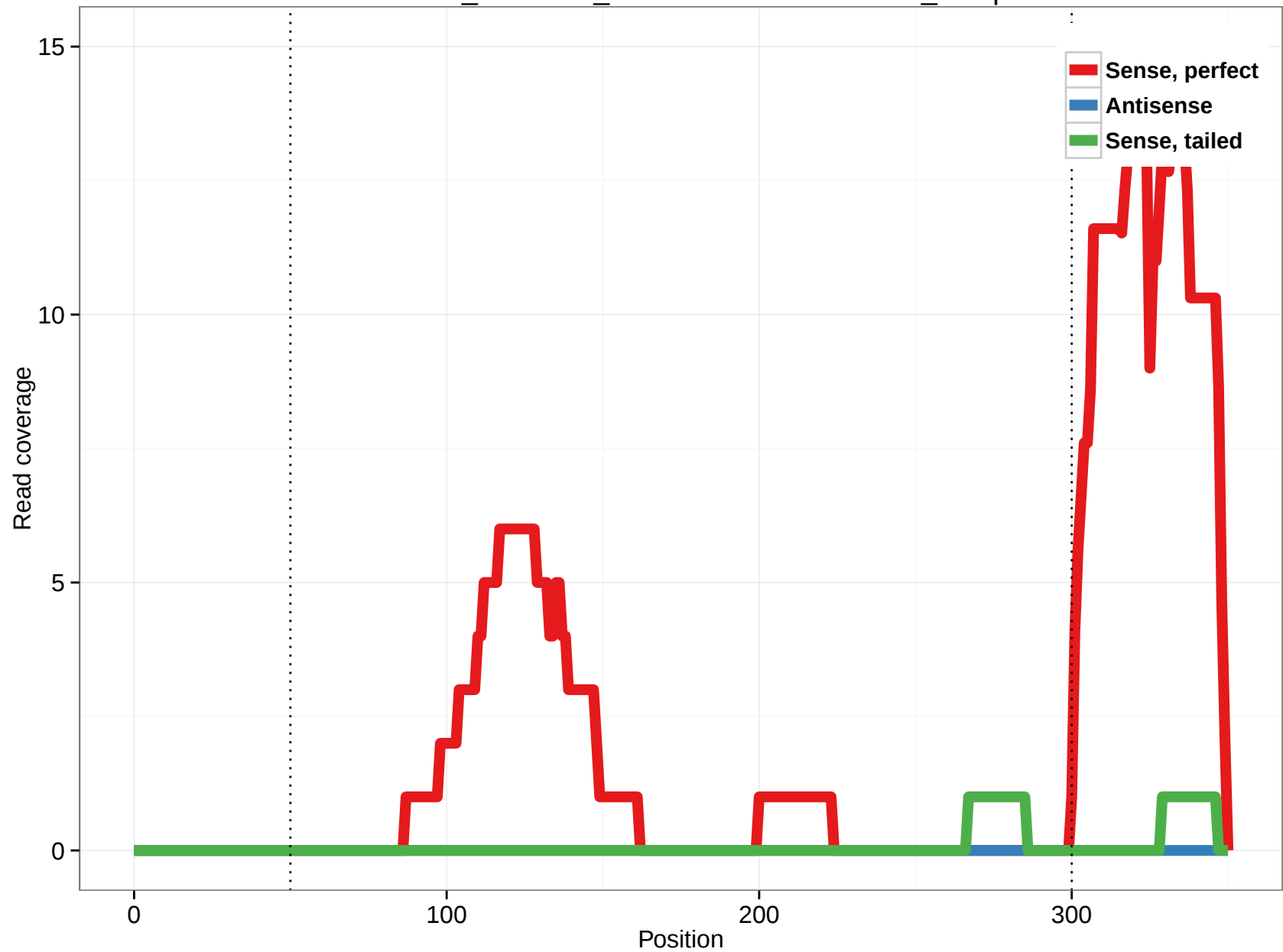
ornAna1_ensGene_ENSOANT00000022276_22.3p
