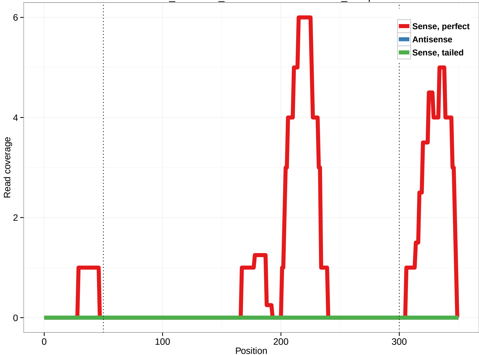
ornAna1_ensGene_ENSOANT00000022276_15.3p
