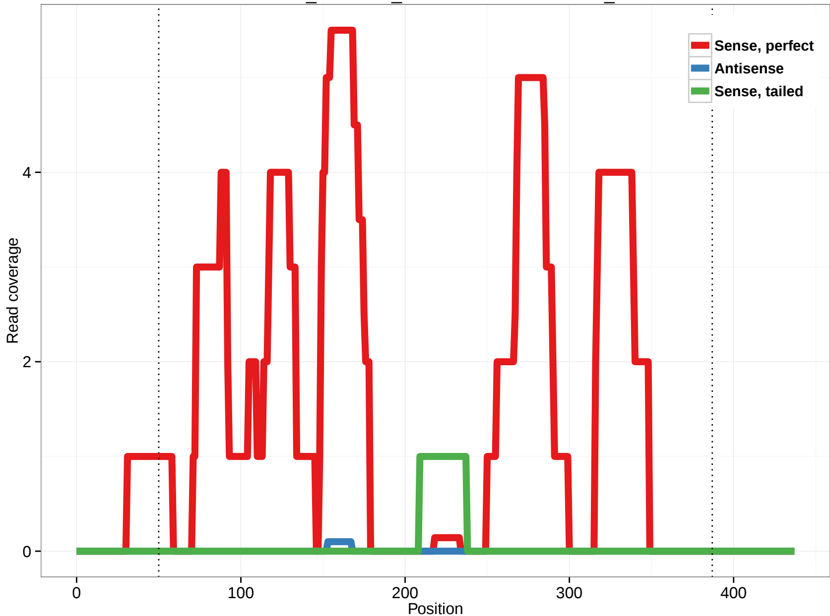
ornAna1_ensGene_ENSOANT00000022257_13
