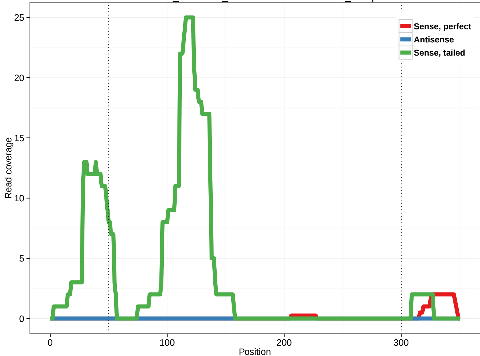
ornAna1_ensGene_ENSOANT00000022254_20.3p
