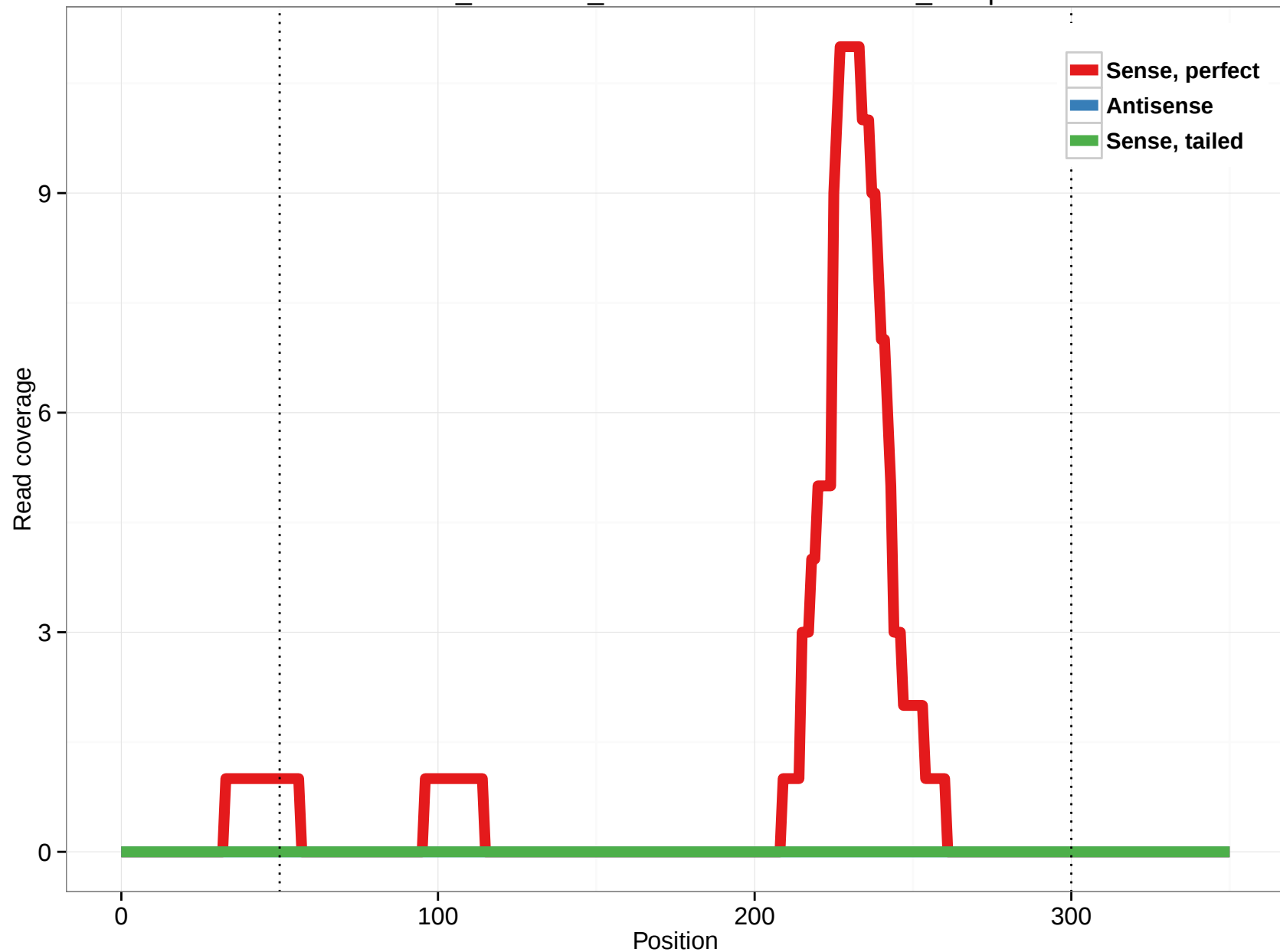
ornAna1_ensGene_ENSOANT00000022180_15.5p
