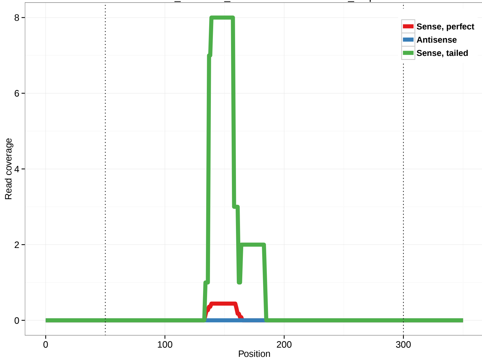
ornAna1_ensGene_ENSOANT00000022179_3.3p
