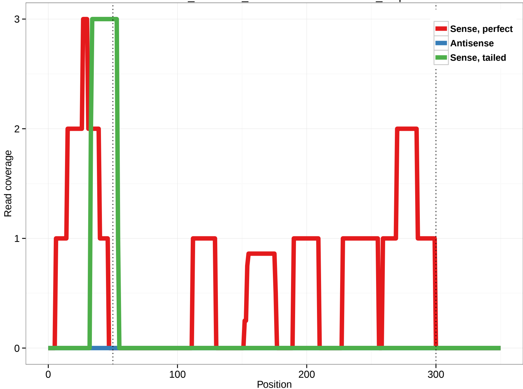
ornAna1_ensGene_ENSOANT00000022090_1.5p
