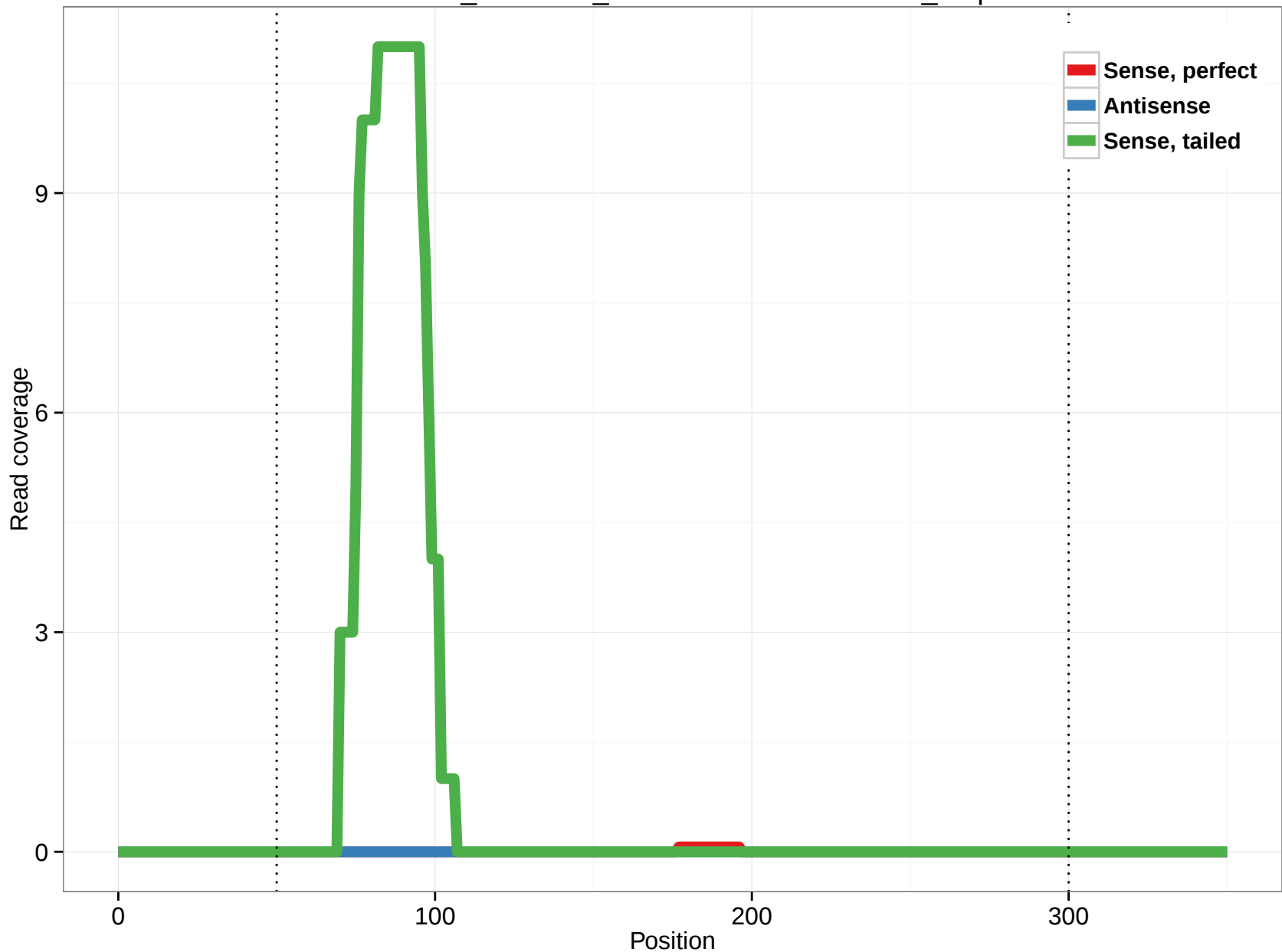
ornAna1_ensGene_ENSOANT00000022082_4.3p
