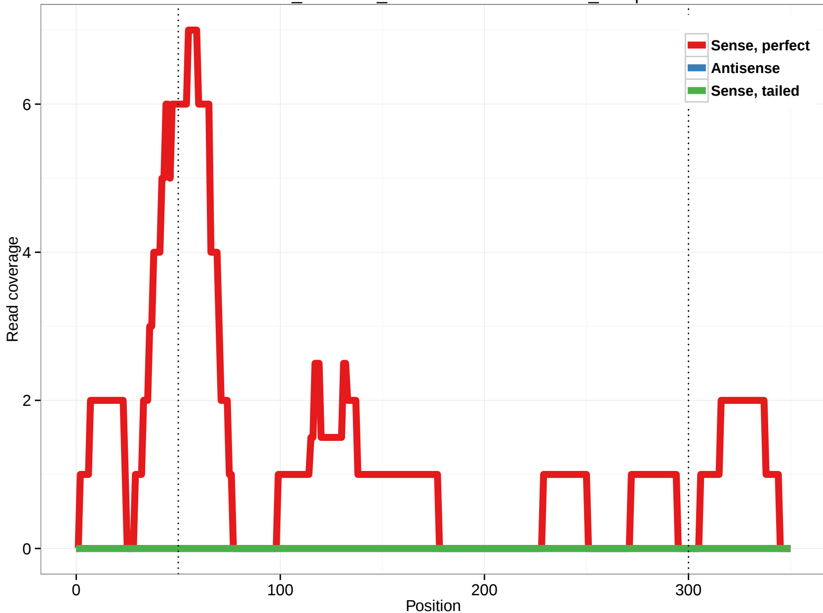
ornAna1_ensGene_ENSOANT00000022058_12.5p
