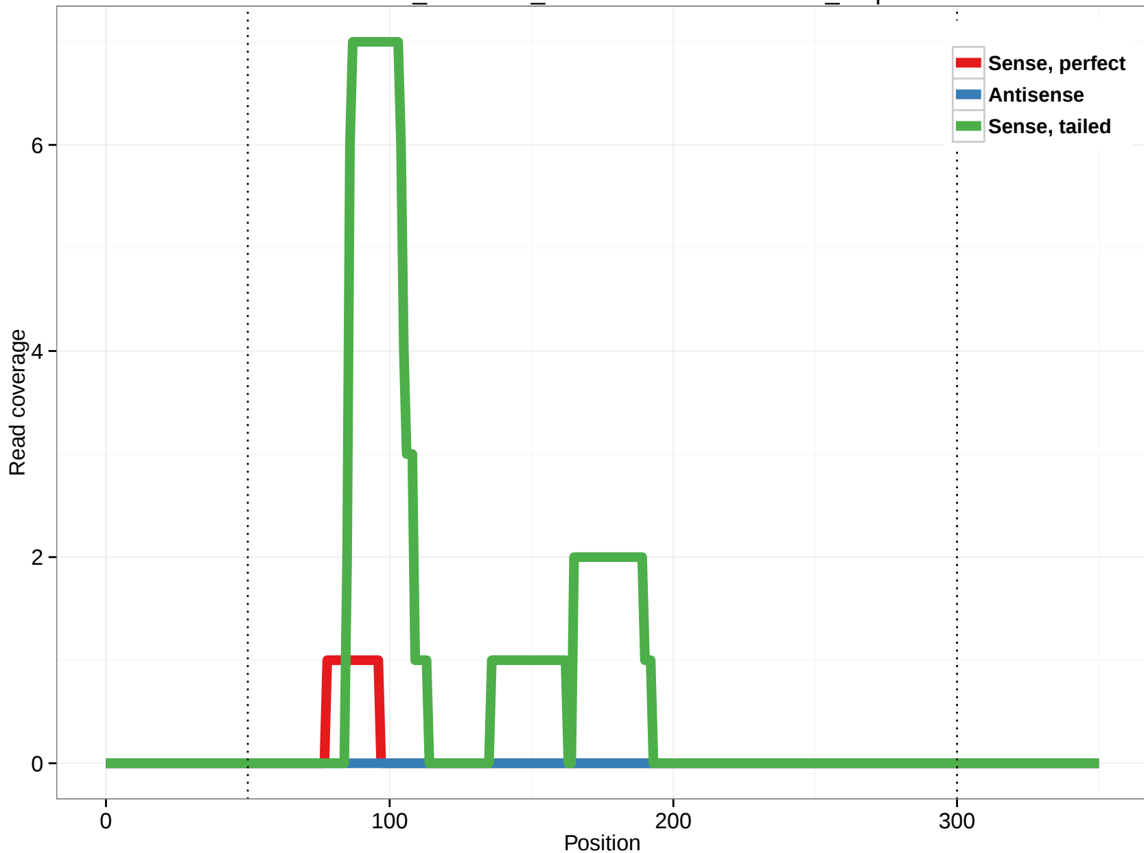
ornAna1_ensGene_ENSOANT00000022042_7.5p
