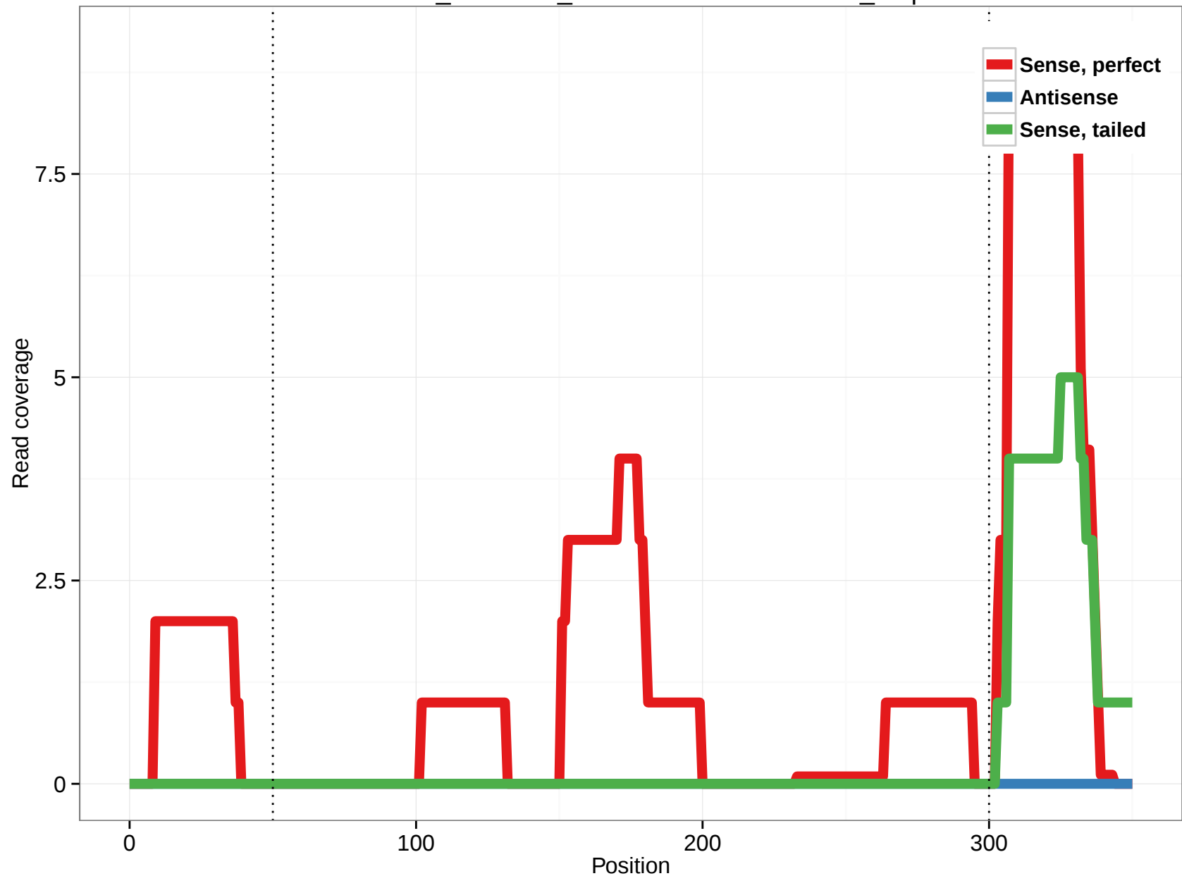
ornAna1_ensGene_ENSOANT00000021979_7.5p
