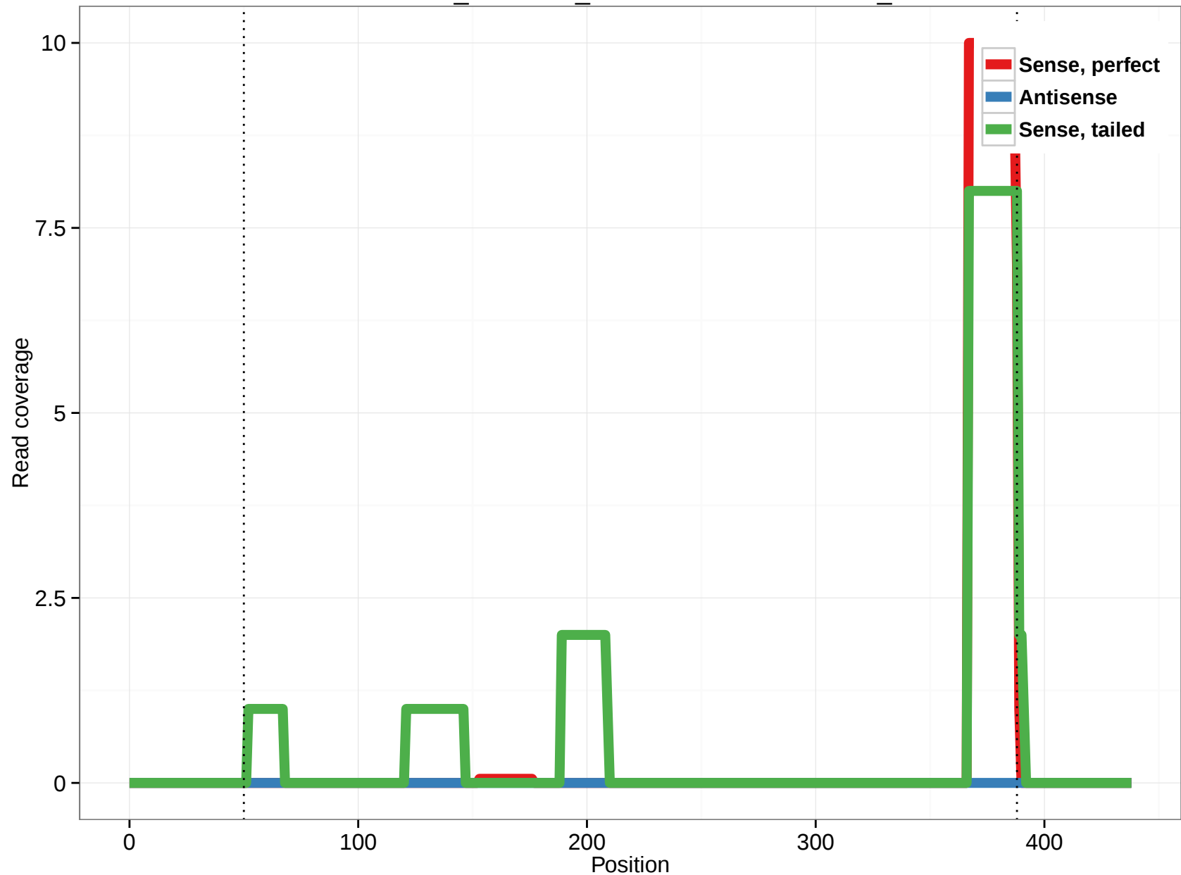
ornAna1_ensGene_ENSOANT00000021923_0
