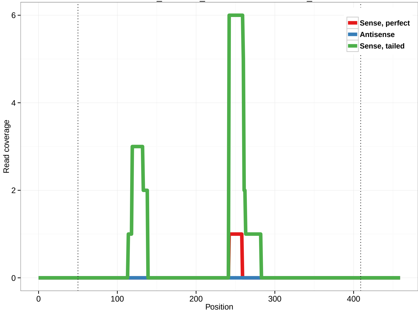
ornAna1_ensGene_ENSOANT00000021900_2
