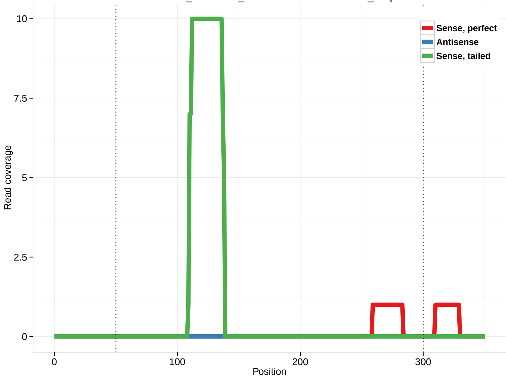
ornAna1_ensGene_ENSOANT00000021897_6.3p
