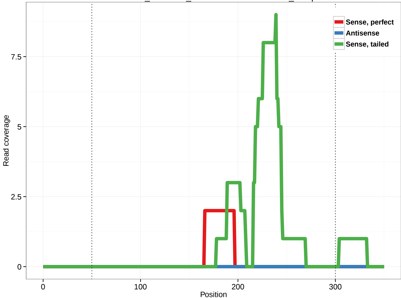
ornAna1_ensGene_ENSOANT00000021893_21.5p
