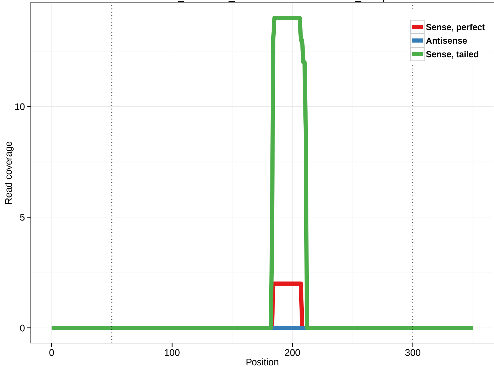
ornAna1_ensGene_ENSOANT00000021888_11.3p
