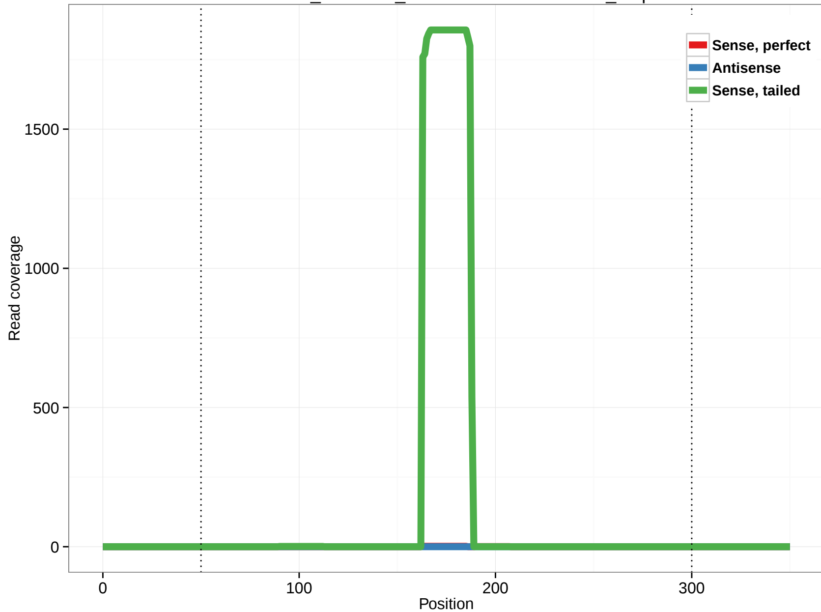
ornAna1_ensGene_ENSOANT00000021834_5.3p
