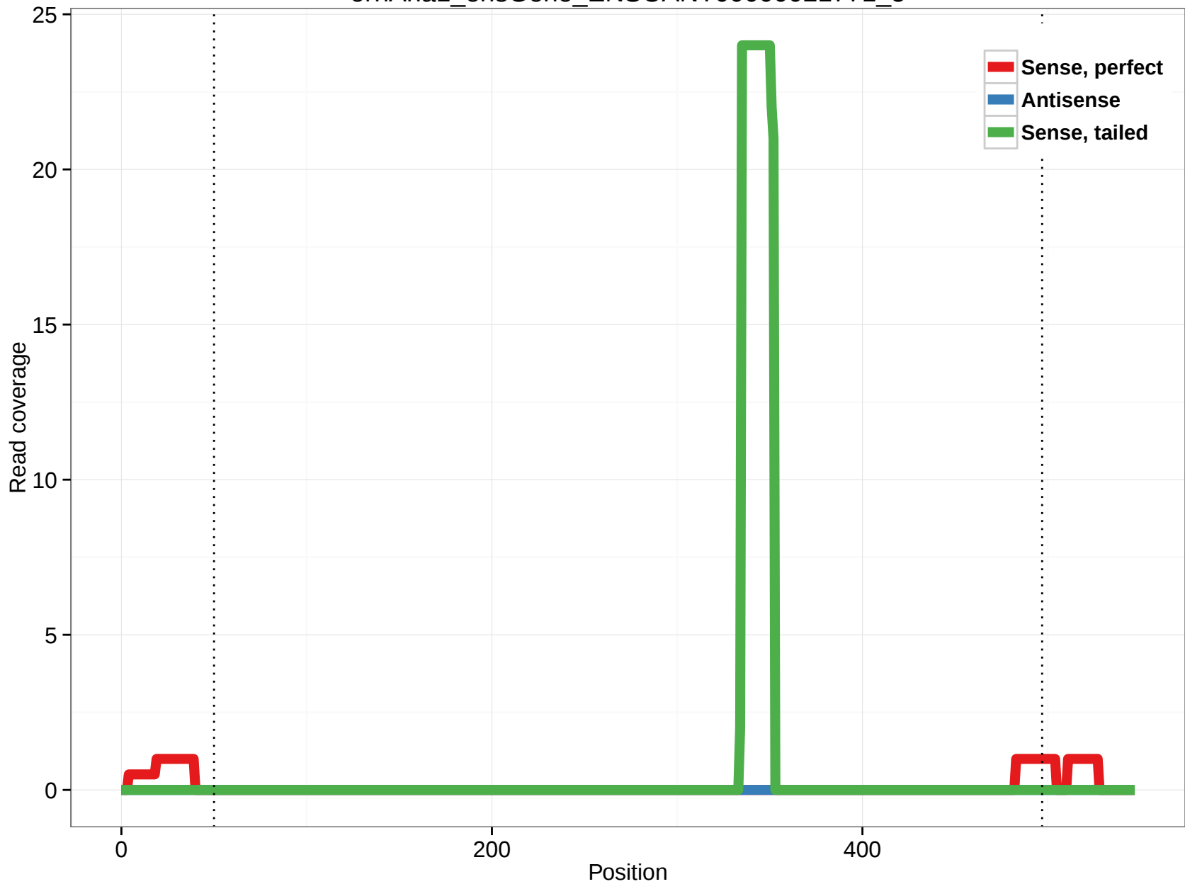
ornAna1_ensGene_ENSOANT00000021771_5
