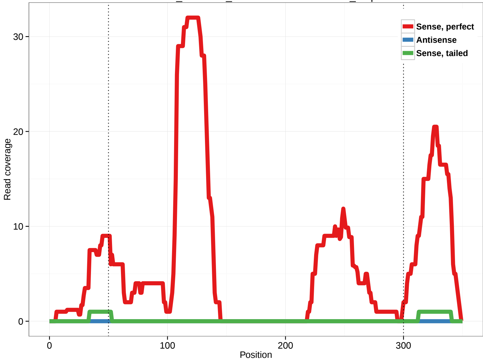
ornAna1_ensGene_ENSOANT00000021750_9.5p
