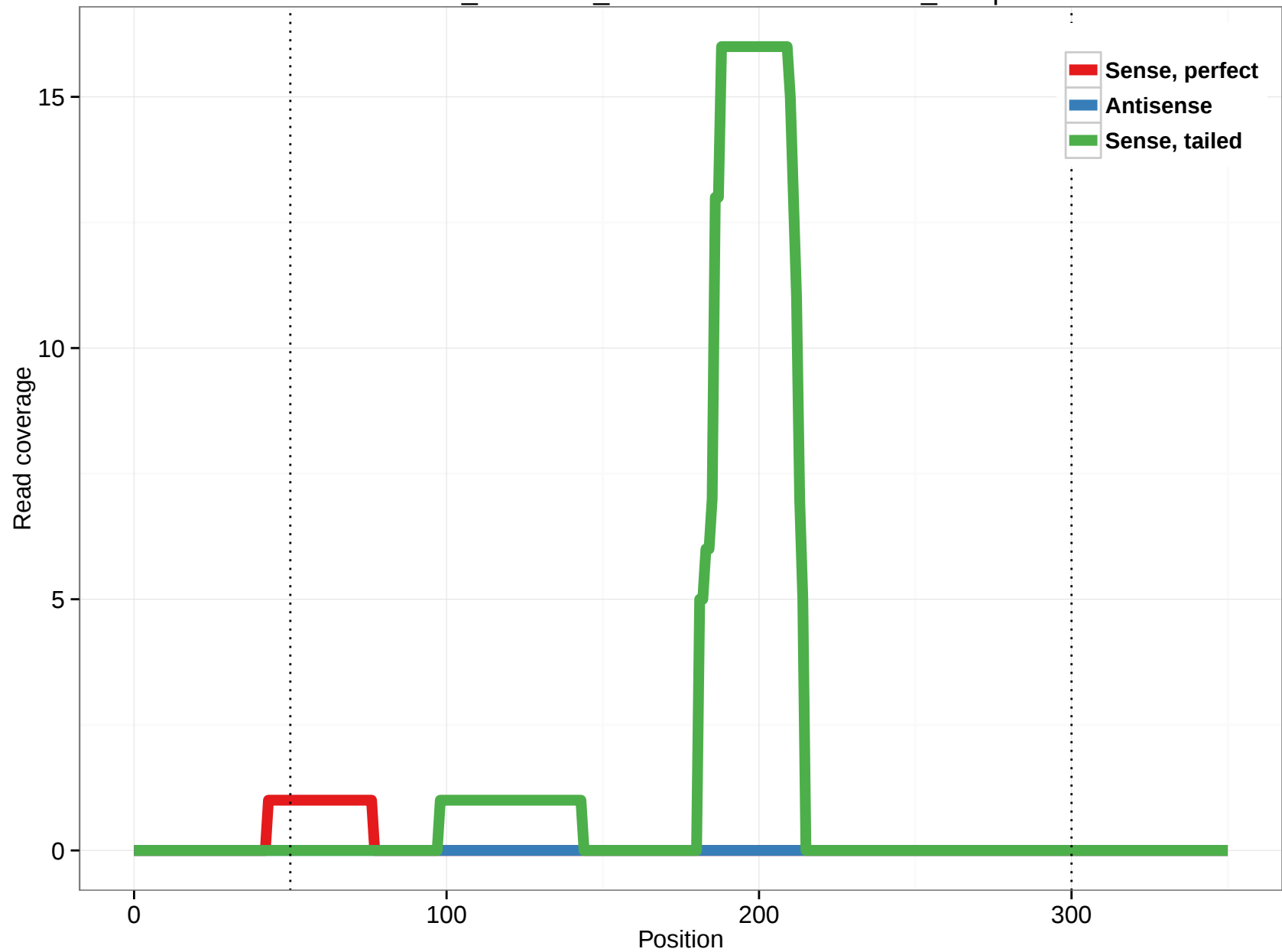
ornAna1_ensGene_ENSOANT00000021550_10.5p
