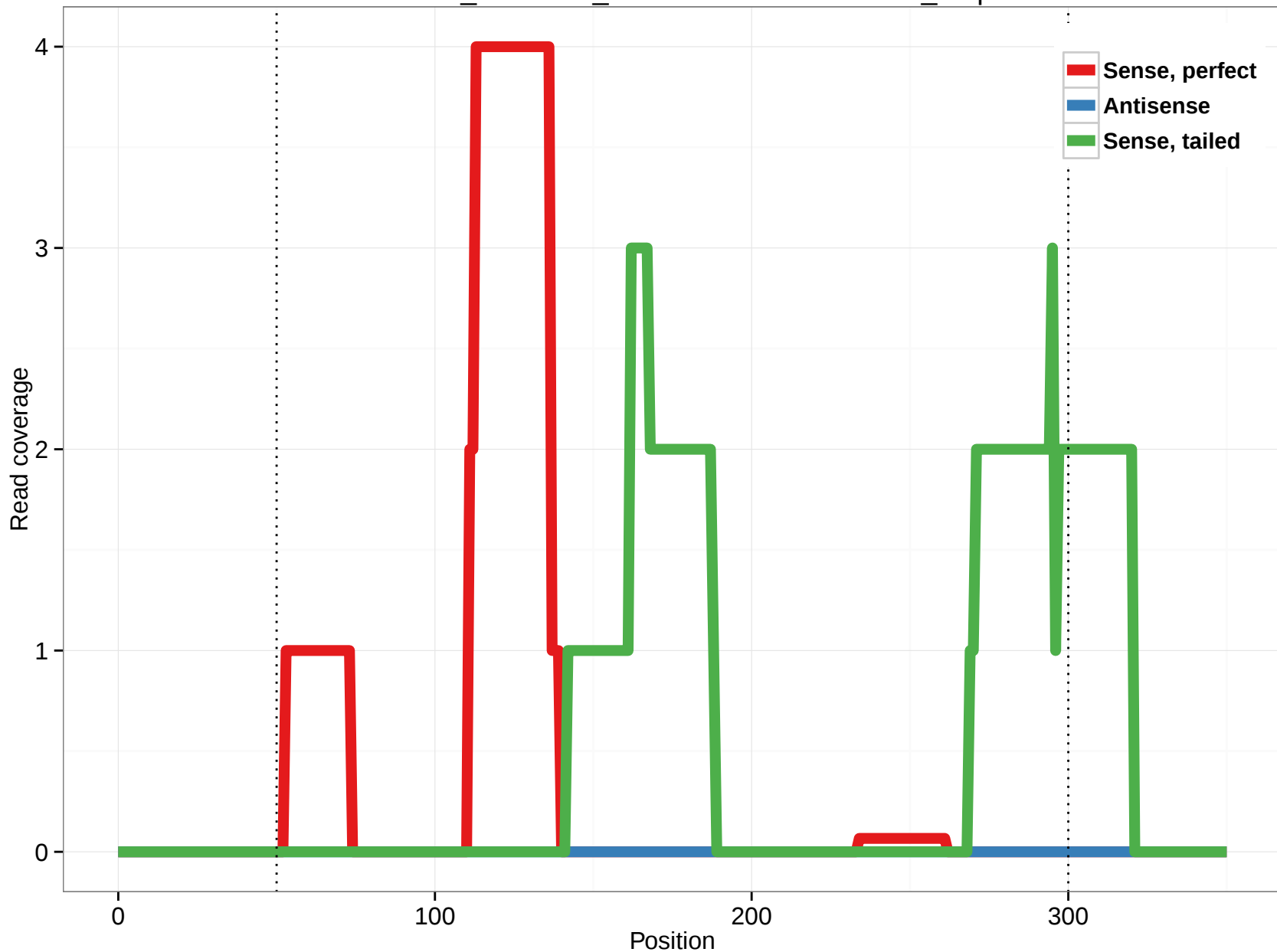
ornAna1_ensGene_ENSOANT00000021544_3.5p
