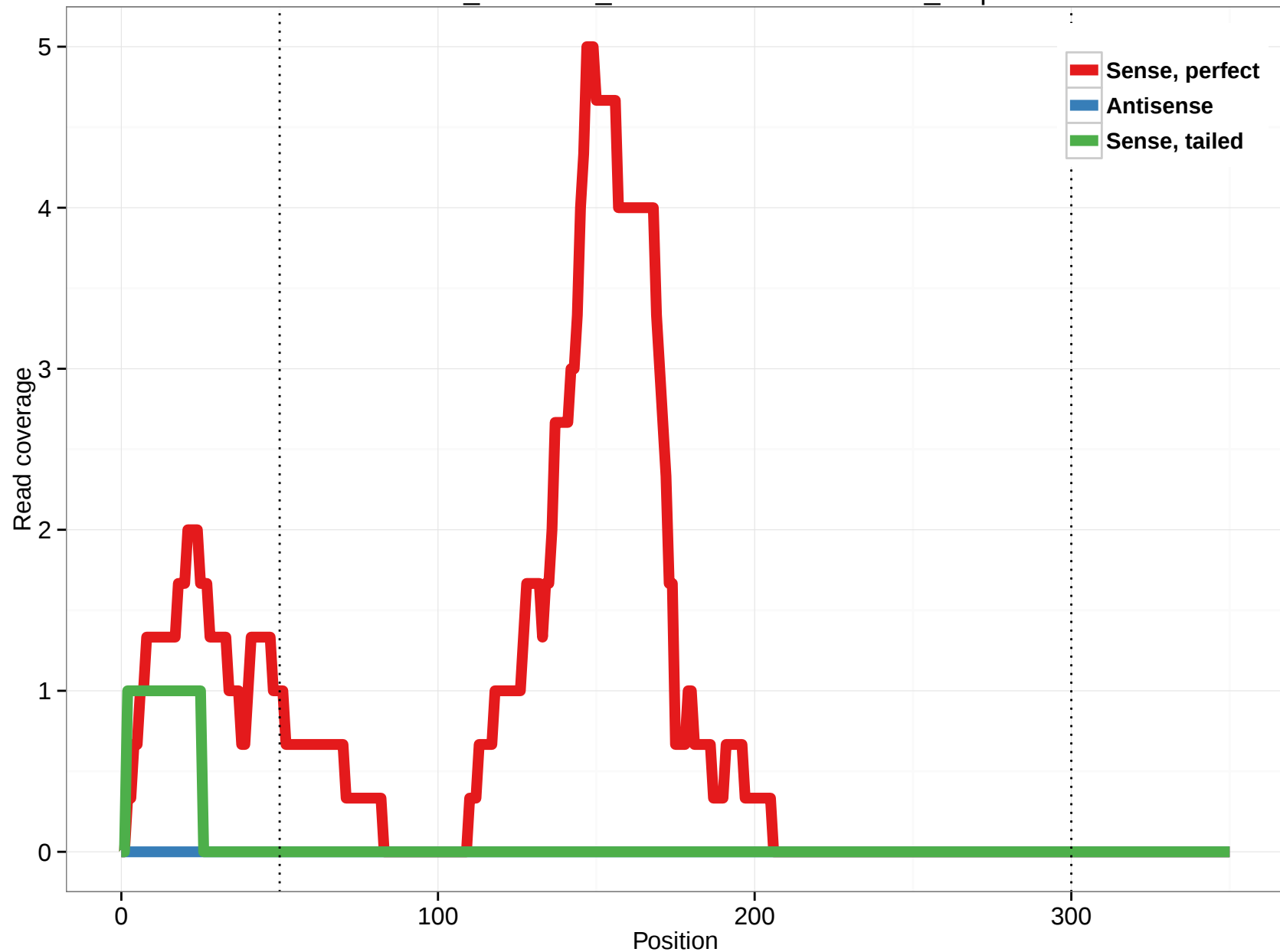
ornAna1_ensGene_ENSOANT00000021534_4.5p
