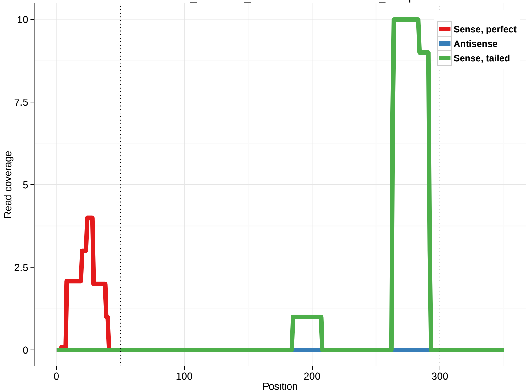
ornAna1_ensGene_ENSOANT00000021434_12.5p
