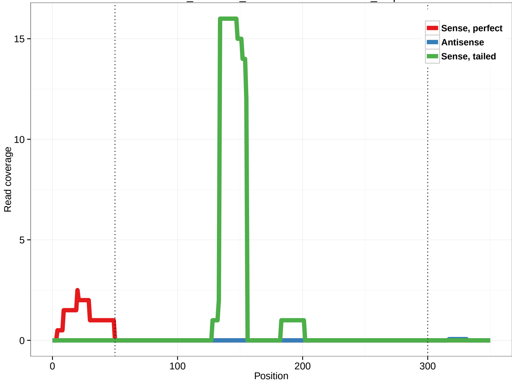
ornAna1_ensGene_ENSOANT00000021360_2.5p
