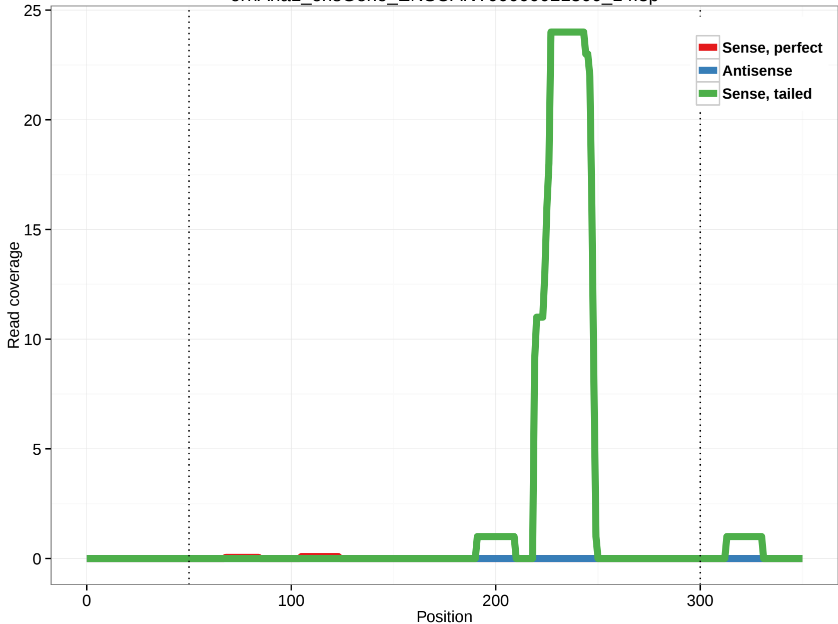
ornAna1_ensGene_ENSOANT00000021300_14.3p
