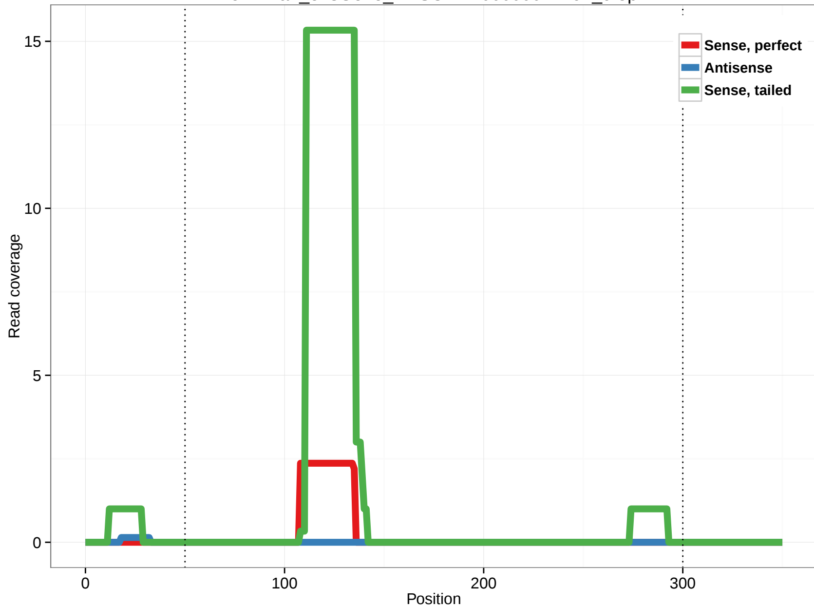
ornAna1_ensGene_ENSOANT00000021294_9.5p
