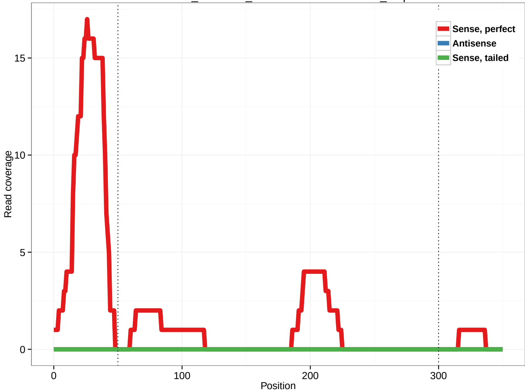
ornAna1_ensGene_ENSOANT00000021288_0.5p
