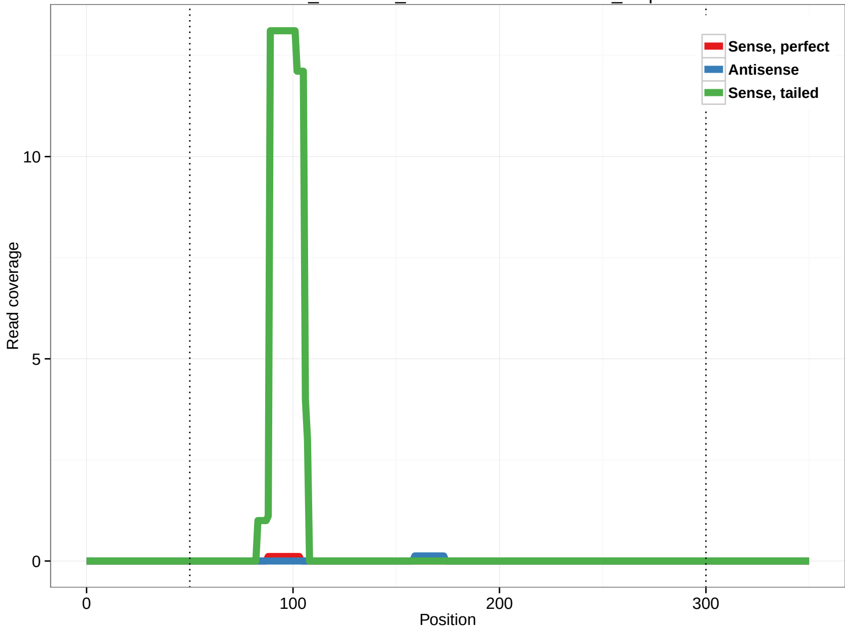
ornAna1_ensGene_ENSOANT00000021264_1.5p
