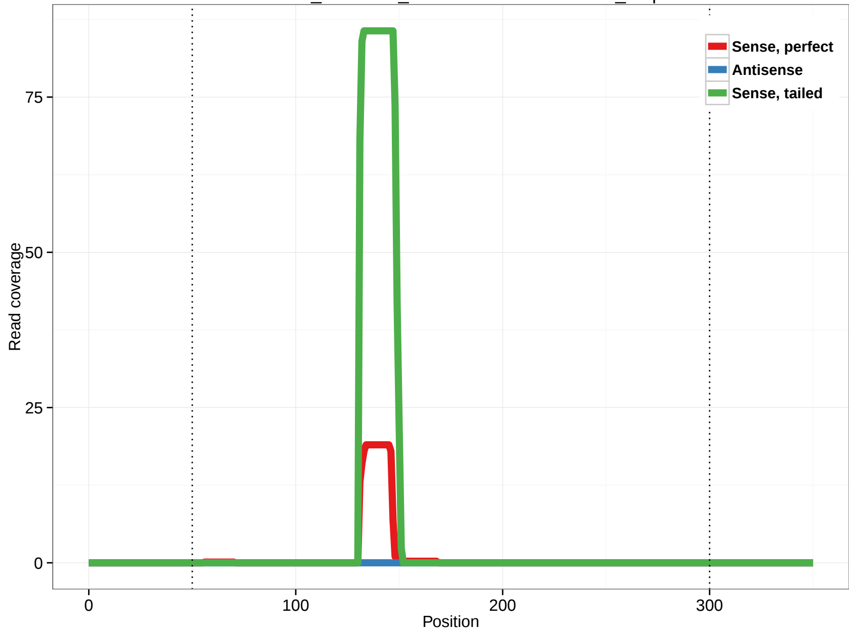
ornAna1_ensGene_ENSOANT00000021247_8.3p
