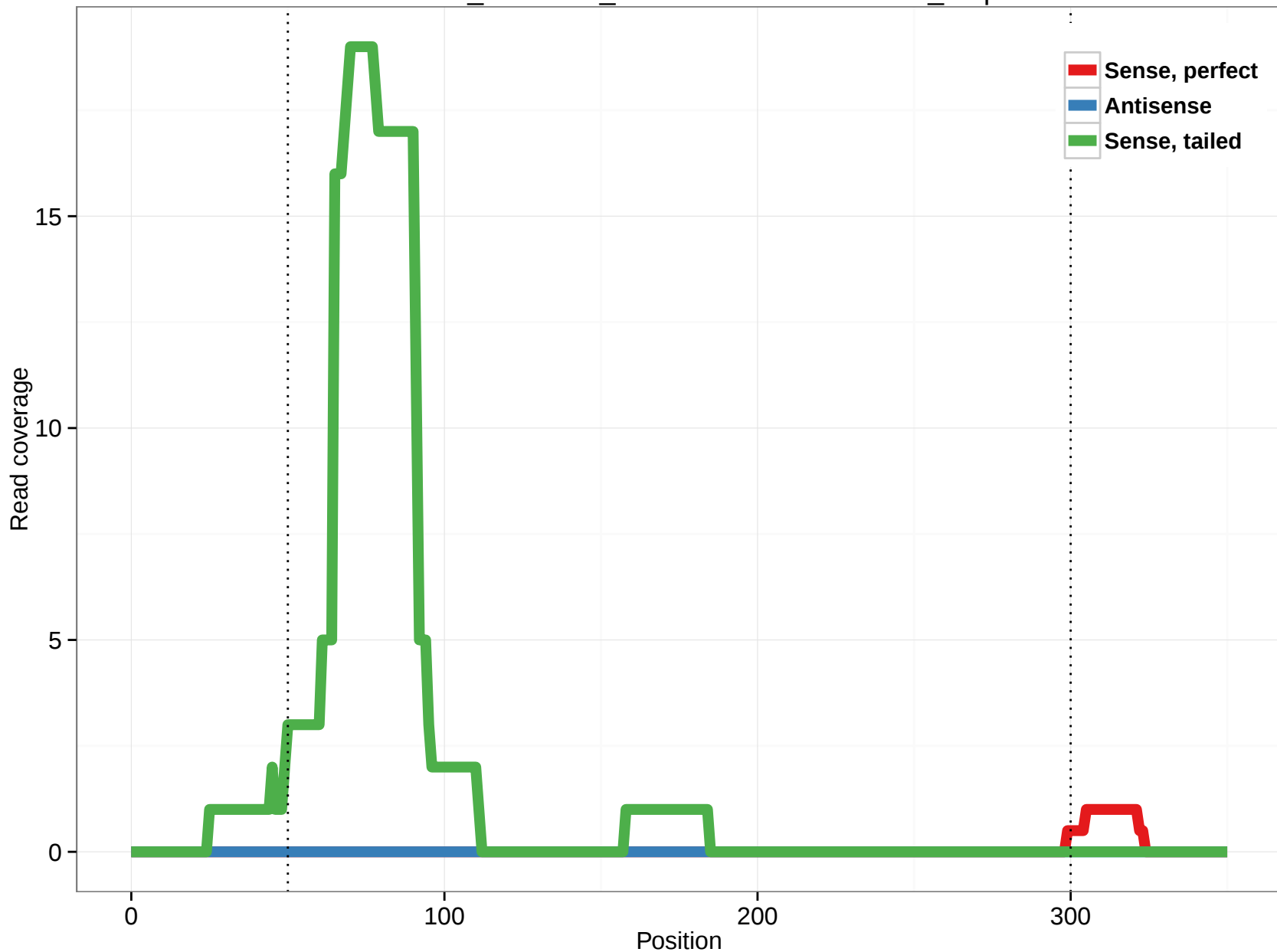
ornAna1_ensGene_ENSOANT00000021230_2.3p
