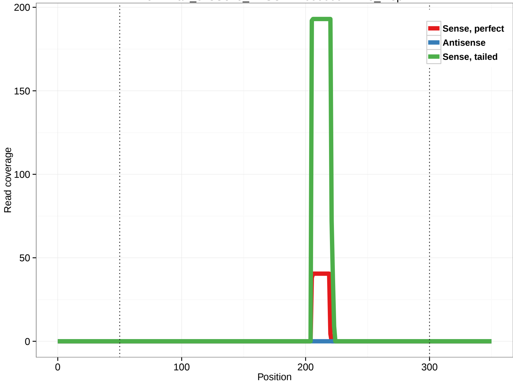
ornAna1_ensGene_ENSOANT00000021225_4.3p
