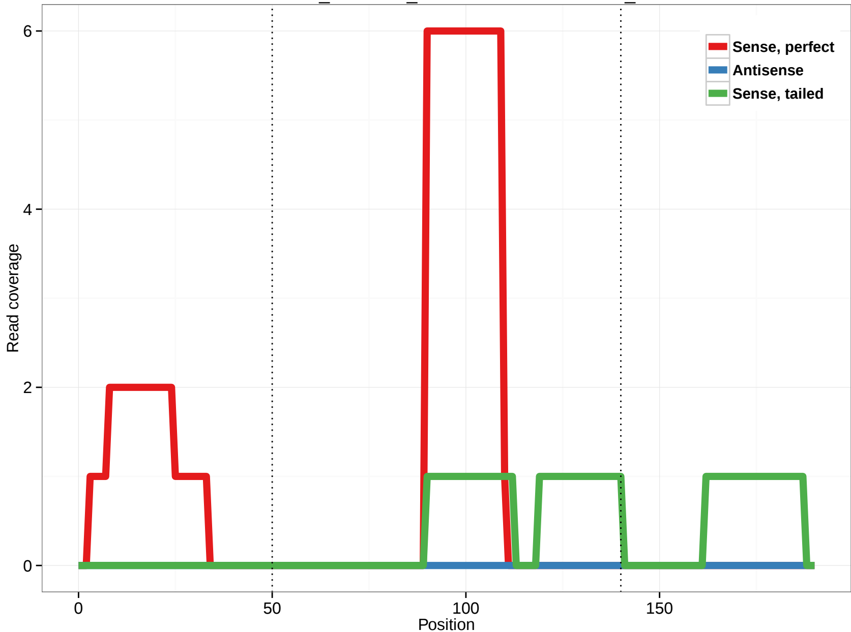
ornAna1_ensGene_ENSOANT00000021190_5
