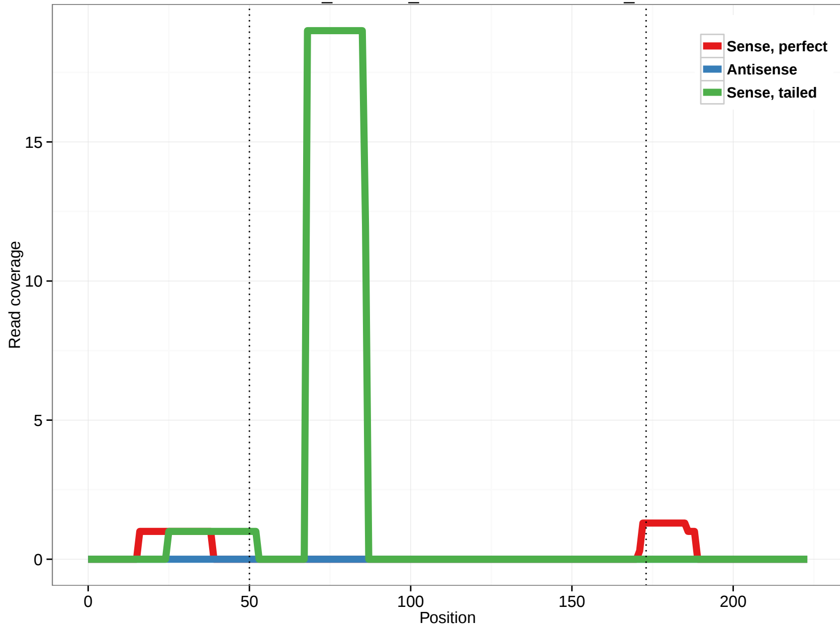
ornAna1_ensGene_ENSOANT00000021138_4
