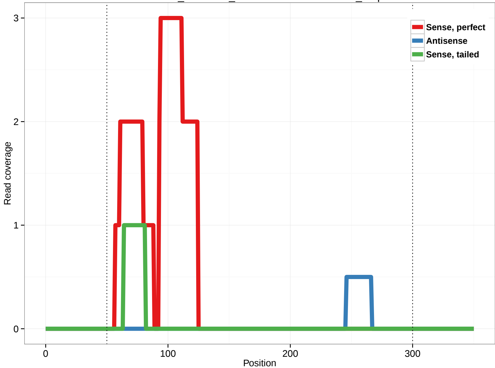
ornAna1_ensGene_ENSOANT00000021131_6.5p
